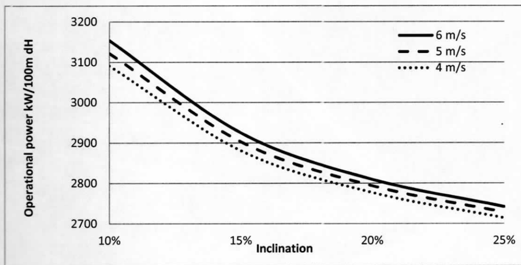
Figure 4. Power demand for 100 m lifting at 10 000 t/h
