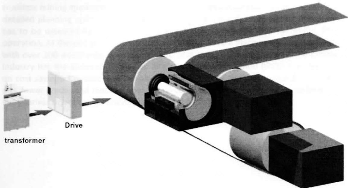
Figure 7. Principle of direct gearless drive technology (Courtesy: ABB)
